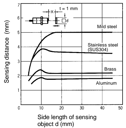
E2EG-X5MCj /Bj
