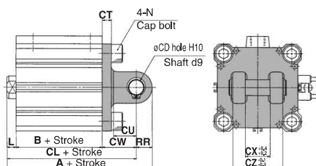
Double clevis style: CQ2D/CDQ2D
