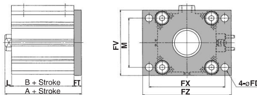
Head side flange style: CQ2G/CDQ2G
